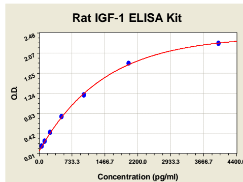
Figure 1: IGF-1 Standard Curve. Using the rat IGF-1 ELISA Kit, O.D. data was graphed against IGF-1 protein concentration. The TMB reaction was incubated at 37°C for 27 min.
